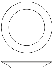
2. prato CH plate CH plato CH assiette CH cod. ref. 08-003 pt.CH ∅ 31
